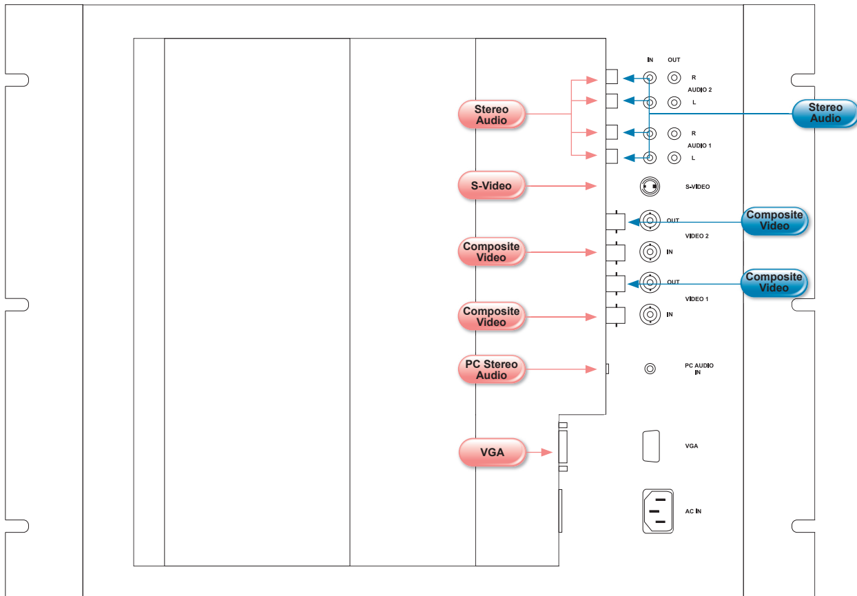
LM-1511R Panel illustrated - LM-1911R has same I/O configuration
